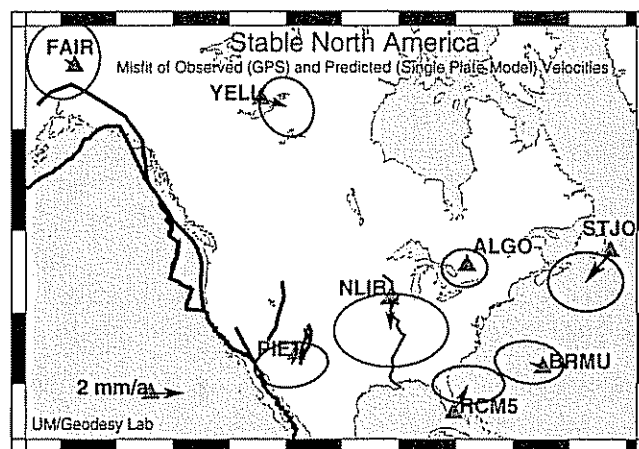
Figure 2. Similar to Figure 1, showing velocity residuals (Table 1) and 95% confidence ellipses. Note scale change.
