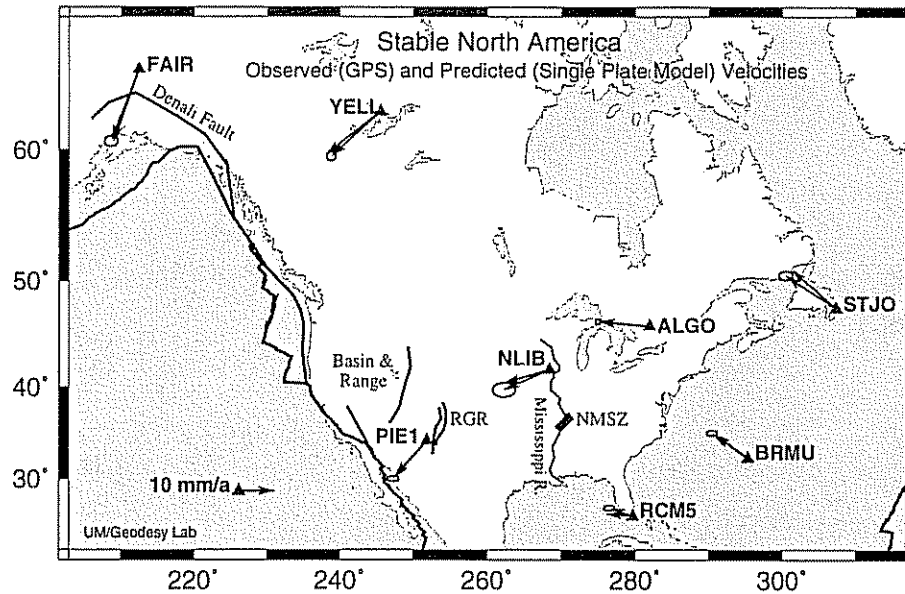
Figure 1. Stations used in this study, their GPS-derived velocities and 95% confidence ellipses, and their velocities predicted by the single rigid plate model in Table 1 (arrows with no ellipse). Major tectonic features discussed in text are also shown. RGR is Rio Grande Rift; NMSZ in New Madrid Seismic Zone.
