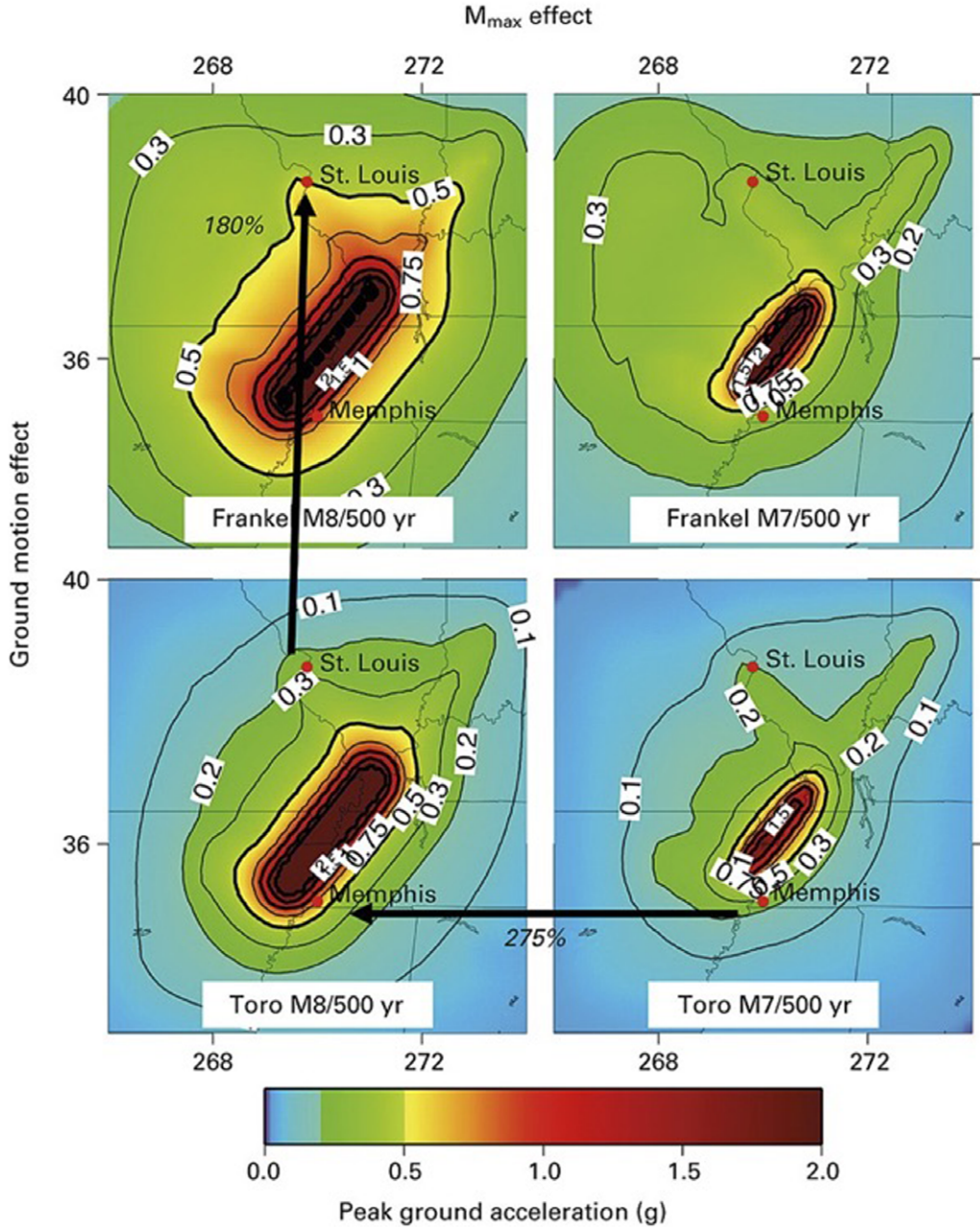
Fig. 14. Comparison of different hazard maps (2% probability in 50 years) for the New Madrid seismic zone (Newman et al. 2001).
