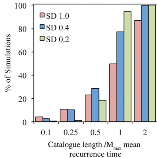
Fig. 10. Numerical simulations assessing how well earthquake catalogues of different lengths recover the actual maximum magnitude M_{\max} of earthquakes in an area. Catalogue lengths are given as a fraction of the mean recurrence time for earthquakes with magnitude M_{\max} . Colours show results for Gaussian distributions of recurrence times with standard deviation equal to the indicated fraction of the mean. The largest earthquake observed probably reflects the length of the history used, even if larger earthquakes occur, so a catalogue shorter than an earthquake’s mean recurrence time is likely to not contain an event of that size (Stein & Friedrich 2014; Merino 2014). Reproduced with permission of the Royal Astronomical Society.
