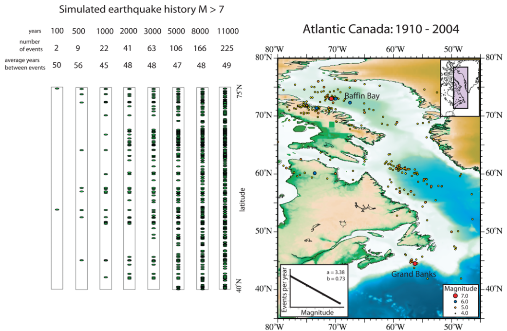
Fig. 9. Intraplate seismicity along the eastern coast of Canada. Simulations using a frequency–magnitude relation derived from these data predict that if seismicity is uniform in the zone, about 11 000 years of record is needed to avoid apparent concentrations and gaps (Swafford & Stein 2007). Reproduced with permission of Geological Society of America.
