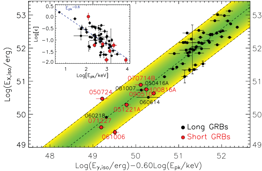
Figure 10. Three-parameter correlation involving E_{X, \text{iso}} , E_{\gamma, \text{iso}} and E_{\text{pk}} . Dashed line: best-fitting relation (equation 8); dot-dashed lines: the 95 per cent confidence area around the best-fitting law. Notably, long and short GRBs share the same scaling, with short and sub-energetic GRBs (like GRB 060218) occupying the same area of the plot. Inset: evolution of the efficiency parameter \epsilon \equiv E_{X, \text{iso}}/E_{\gamma, \text{iso}} as a function of the spectral peak energy of the prompt emission E_{\text{pk}} . A reference \epsilon \propto E_{\text{pk}}^{-0.6} scaling has been marked with a blue dashed line.
