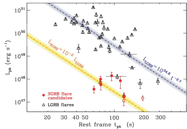
Figure 3. 0.3–10 keV peak luminosity evolution with time for LGRB flares (black open triangles, from Chincarini et al. 2010) and SGRB flare candidates with and without extended emission (red open and filled circles, respectively). Blue dashed line: best-fitting power-law model for LGRB flares: L_{\text{pk,F}}^{\text{LGRB}} = 10^{54.8 \pm 0.4} [t_{\text{pk}}/(1+z)]^{-2.7 \pm 0.5} and intrinsic scatter \sigma = 0.73 \pm 0.08 . Orange dot-dashed line: best-fitting L_{\text{pk,F}}^{\text{LGRB}} decay renormalized by a factor of 100 to match the observed SGRB flare candidates L_{\text{pk,F}}^{\text{SGRB}} .
