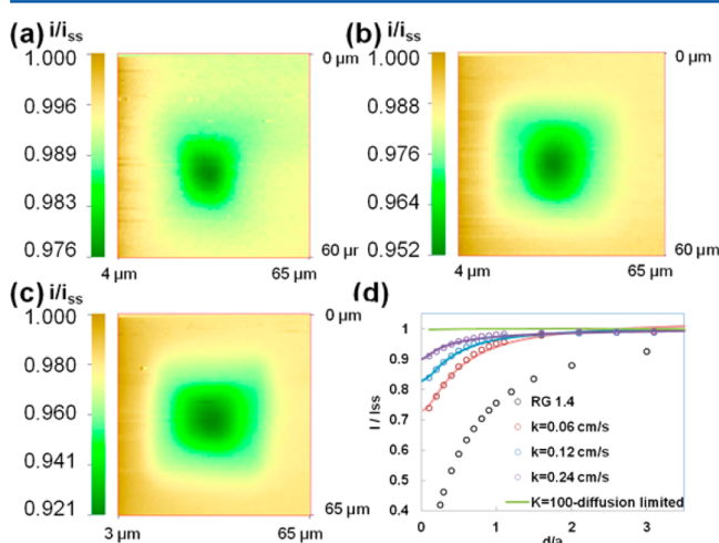
Figure 5. Representative SECM images of microchambers with FcMeOH permeabilities of (a) 0.24, (b) 0.12, and (c) 0.06 cm/s. All the SECM images were measured at 2 \mu\text{m} above the chamber roof with a 2.5 \mu\text{m} radius Pt UME with RG 1.4. The current values are normalized by the limiting current in the bulk solution, I_{ss} . (d) SECM approach curves obtained over the chamber roof for each condition. The permeability to FcMeOH is estimated by fitting the experimental data with finite element simulation.
