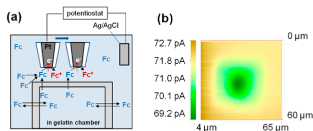
Figure 4. (a) SECM cell with the 3D printed protein microchamber filled with 0.1 mM FcMeOH and MOPS buffer solution. The Pt UME positioned at a constant height of 2 \mu\text{m} above the chamber roof is biased at 0.4 V vs Ag/AgCl to oxidize FcMeOH. (b) SECM image over the chamber in the FcMeOH solution produced by scanning the tip in the x – y direction. The brown color on the current scale represents the highest oxidative current while the green color is the minimum. Tip potential, 0.4 V vs Ag/AgCl. Tip scan rate, 10 \mu\text{m/s} . Pt UME with a = 2.5 \mu\text{m} with RG 1.4 was used for the oxidation of FcMeOH during the SECM image.
