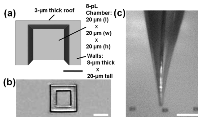
Figure 1. (a) Schematic of a cut-out front view of the 3D printed microchamber designed for SECM studies. The 8 pL inner chamber is 20 \times 20 \times 20 \mu m ( l \times w \times nominal height), and the outer dimensions are 36 \times 36 \times 23 \mu m ( l \times w \times nominal height). The 8 pL chamber is a closed system that is anchored directly to a coverglass surface on the bottom and then surrounded by four, 8 \mu m thick walls and a 3 \mu m thick roof composed of photo-cross-linked protein. Scale bar, 10 \mu m. (b) Bright-field image of the microchamber. The 3 \mu m thick roof is optically transparent and not visible in the image. Scale bar, 20 \mu m. (c) Video-microscope image of a 5 \mu m diameter SECM tip positioned adjacent to an 8 pL 3D printed protein microchamber. Scale bar, 100 \mu m.
