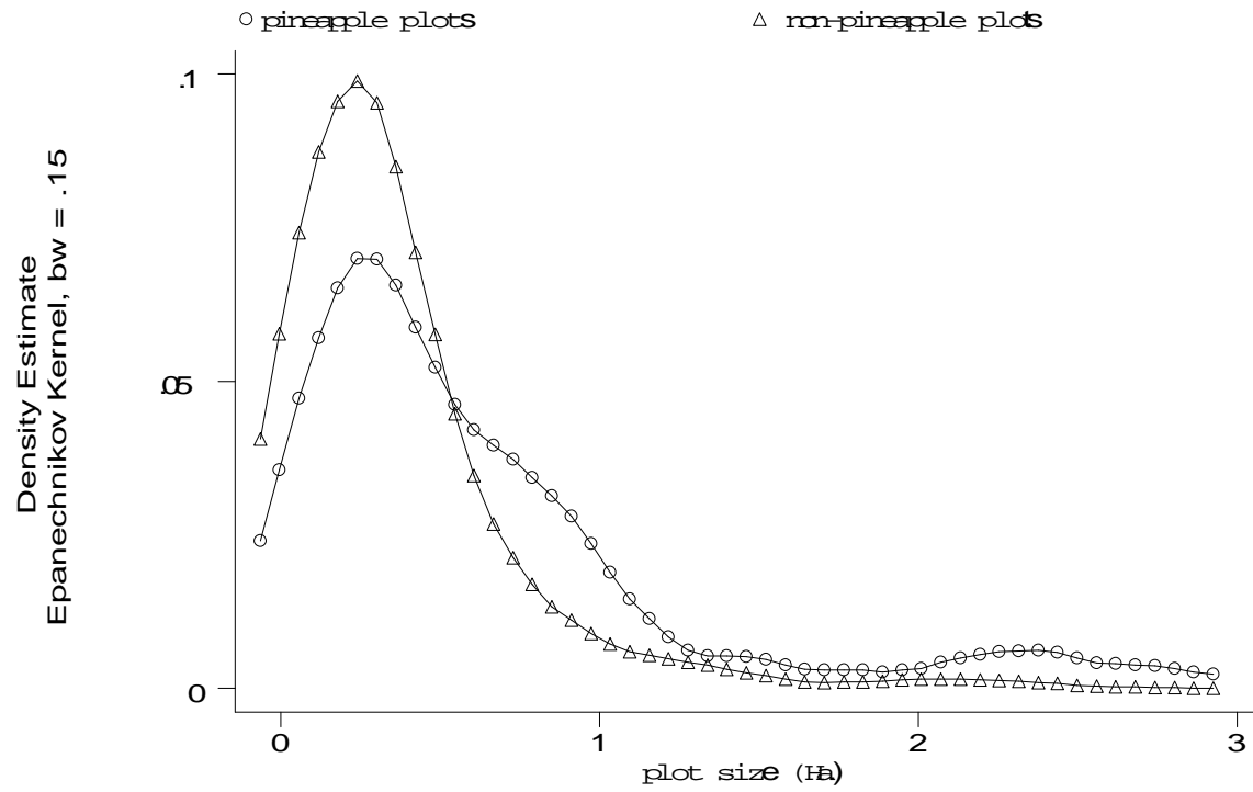
Figure 5: Density of Plot Sizes
